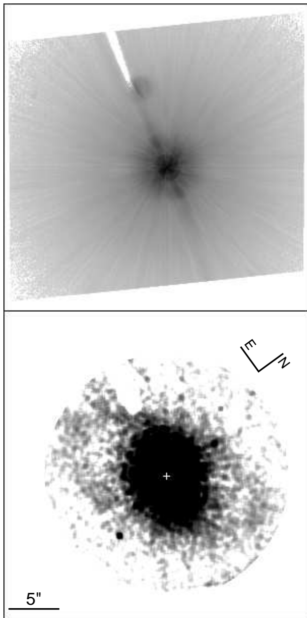
Fig. 1.— ACS F606W coronagraphic observations of HD 207129. Each frame is 30''.2 on a side. (TOP) Coronagraphic image from the first orientation prior to PSF subtraction. Shadows of the occulting finger and larger occulting spot are seen towards the upper left corner. The diagonal streak stretching from the upper left to lower right is instrumentally-scattered light. This image is displayed with logarithmic intensity scaling. (BOTTOM) Image of the HD 207129 ring after applying the iterative roll subtraction method described in the text to the exposures taken at each orientation. The images were rebinned to 0''.1 sampling prior to processing, and the result was additionally smoothed using a median filter. This image is displayed with a quarter-root intensity scaling with a much lower maximum value compared to the top image.
