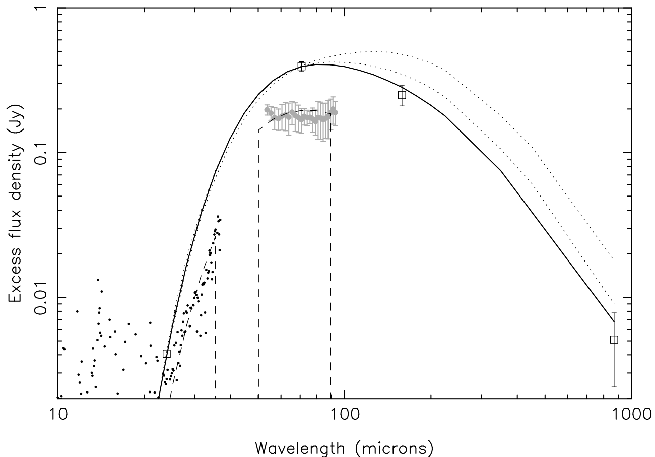
Fig. 5.— Infrared excess of HD 207129 (points), compared to our preferred disk model (solid line) and the disk model windowed by the IRS and MIPS SED slits (dashed lines). The stellar photosphere emission has been removed using a Rayleigh-Jeans slope normalized to the IRS SL data. Relative to Fig. 4, the excess flux densities measured in the IRS and MIPS SED spectra have been reprocessed to remove the point source slit loss correction. The effects of changing the dust size distribution slope from -3.5 (upper dotted curve) to -3.7 (lower dotted curve) to -3.9 (solid curve) are shown. All of the models have the modified albedo.
