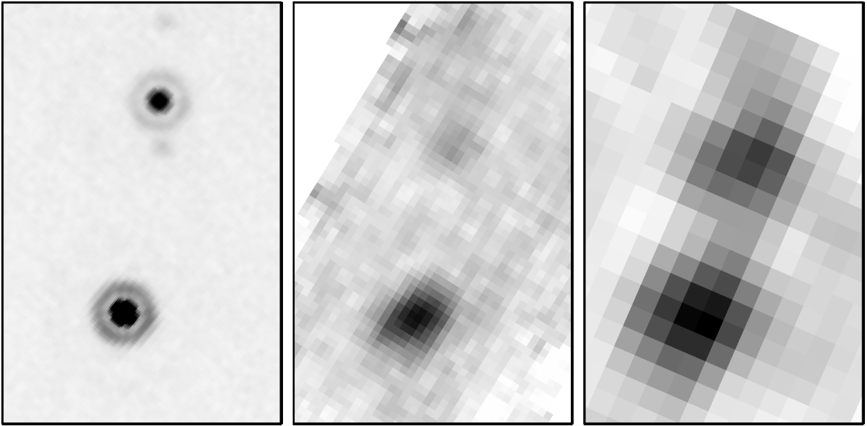
Fig. 3.— Spitzer MIPS images of HD 207129 (lower center), from left to right at 24, 70, and 160 \mu\text{m} respectively. The field of view is 100'' \times 150'' , with N up and E to the left. The 24 \mu\text{m} image is shown in log stretch, while the 70 and 160 \mu\text{m} images are in linear stretch. Only the 70 \mu\text{m} fine scale image is shown. The spectral leak has been subtracted from the 160 \mu\text{m} image shown. The star CD-47 13929 is seen 75'' N of HD 207129 at 24 \mu\text{m} . A very red background object is located 59'' N of HD 207129.
