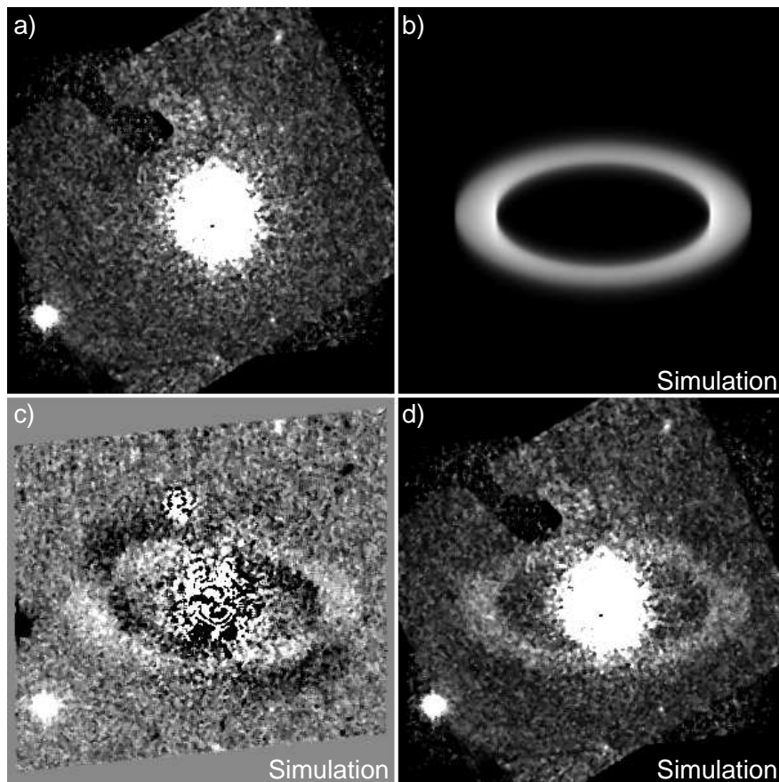
Fig. 2.— Experimental results of applying the roll subtraction algorithm to ACS F606W coronagraphic images of HD 82943 taken at two orientations separated by 25^\circ . Each frame is 30''.2 on a side. (a) Result of the application of the algorithm prior to adding a disk model to the images. The residuals near the center are due to PSF mismatches between the two orientations. (b) Model disk that approximately matches the observed HD 207129 ring. This is added to each HD 82943 image (with a 25^\circ orientation offset in the second image) without noise and with twice the surface brightness of the HD 207129 ring. (c) Direct subtraction of the image from the second orientation from that from the first (with disk models added). Positive and negative images of the ring and background objects are seen. (d) Application of the roll subtraction algorithm to the ring-added images. The resulting ring image appears cleaner than that for HD 207129 because of the increased surface brightness and lack of shot noise in the model.
