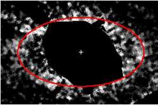
Fig. 6.— The HD 207129 ring ACS image with an ellipse superposed centered on the star (marked by the cross) and having a semi-major axis of 10'' . No large offset of the ring relative to the star, like that seen for Fomalhaut, is seen that would suggest a significant planetary perturber.
