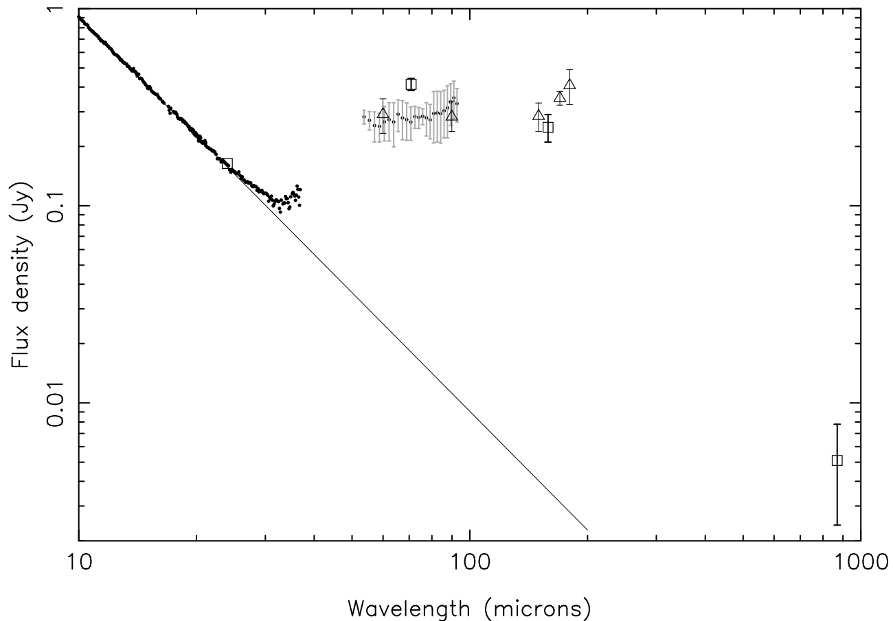
Fig. 4.— Spectral Energy Distribution of HD 207129. Individual data points show the IRS and MIPS SED results, while the three MIPS photometry points are plotted as open squares. ISO measurements appear as open triangles. The solid line shows a Rayleigh-Jeans extrapolation of the stellar photosphere emission based on the IRS data near \lambda = 10 \mu\text{m} . The MIPS-SED spectrum shown here includes a slit loss correction for a point source; therefore, it is low compared to the 70 \mu\text{m} photometry which includes extended emission. The 870 micron point is from Nilsson et al. (2010).
