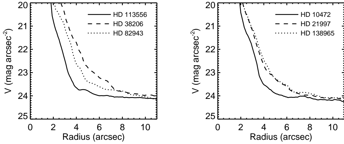
Fig. 8.— Lower limits for the reliable visual detection of a 1'' \times 1'' uniform intensity square around six stars for which no disks were detected.
